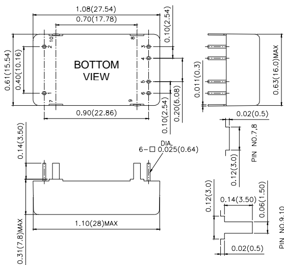
ALL DIMENSIONS IN INCHES (mm) PIN PITCH TOLERANCE ±0.014(0.35)
