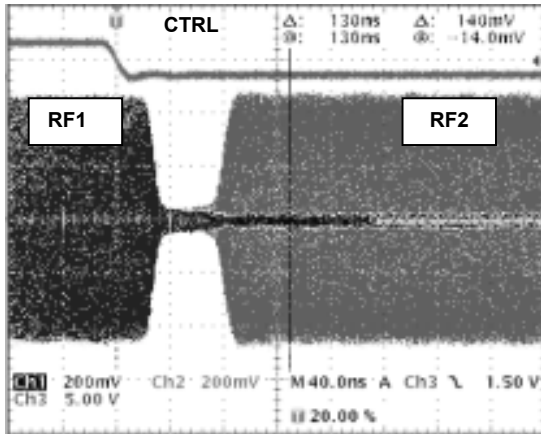
Figure 6. Switching Time
