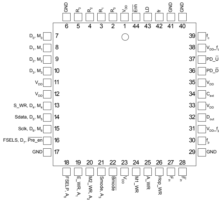
Figure 2. Pin Configuration
