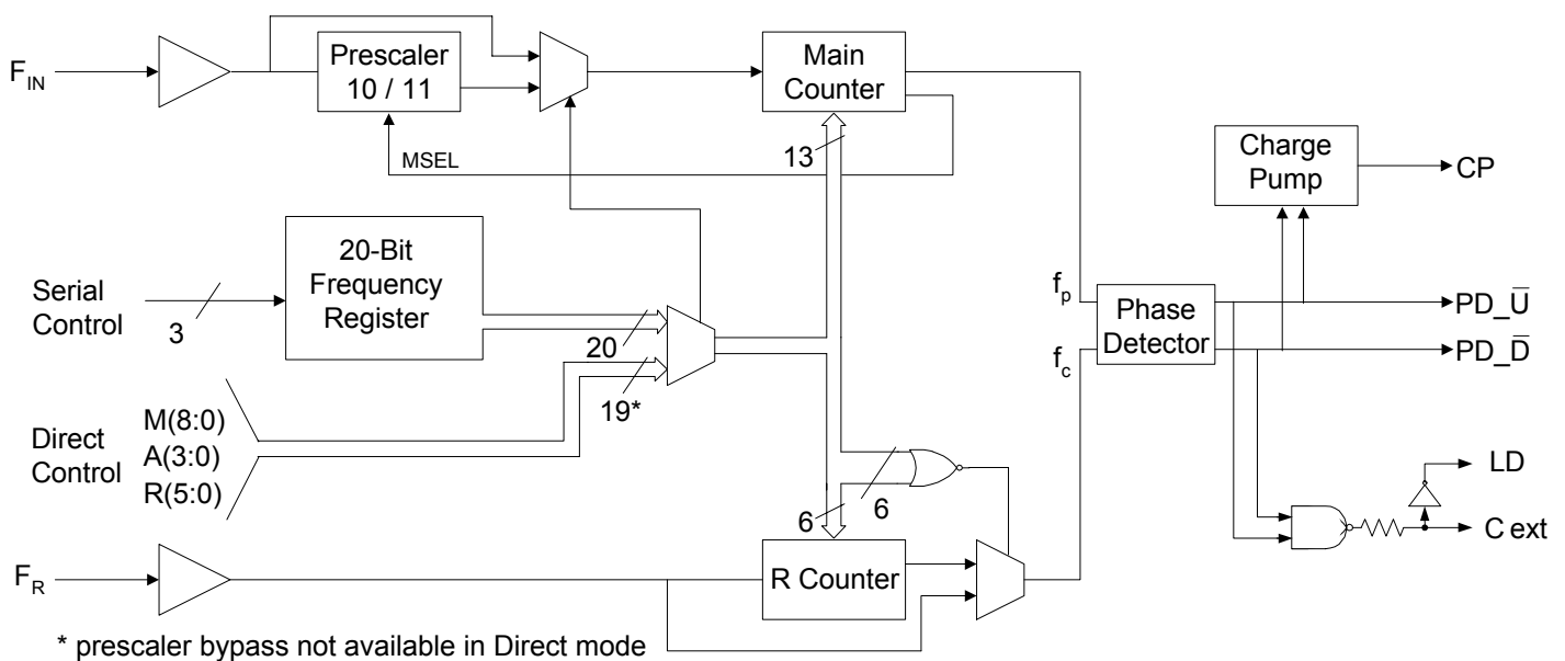
Figure 1. Block Diagram
