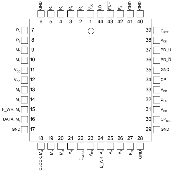
Figure 2. Pin Configuration
