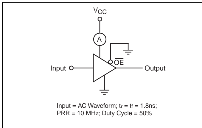
Figure 2. ICCD Test Circuit
