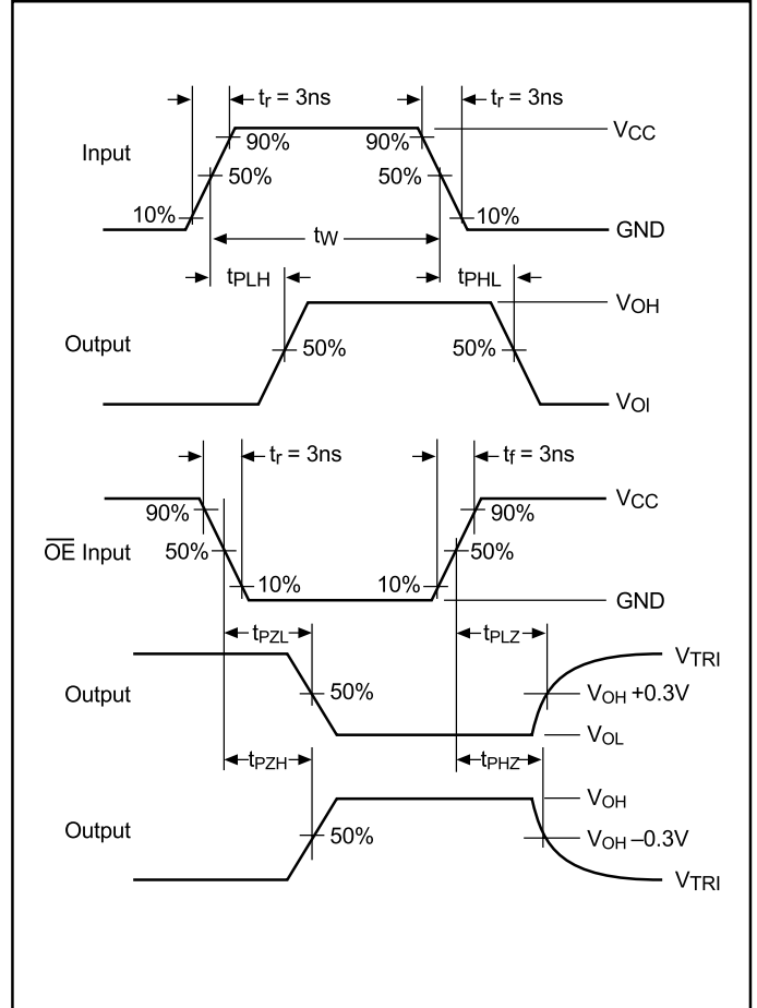
Figure 3. AC Waveforms
