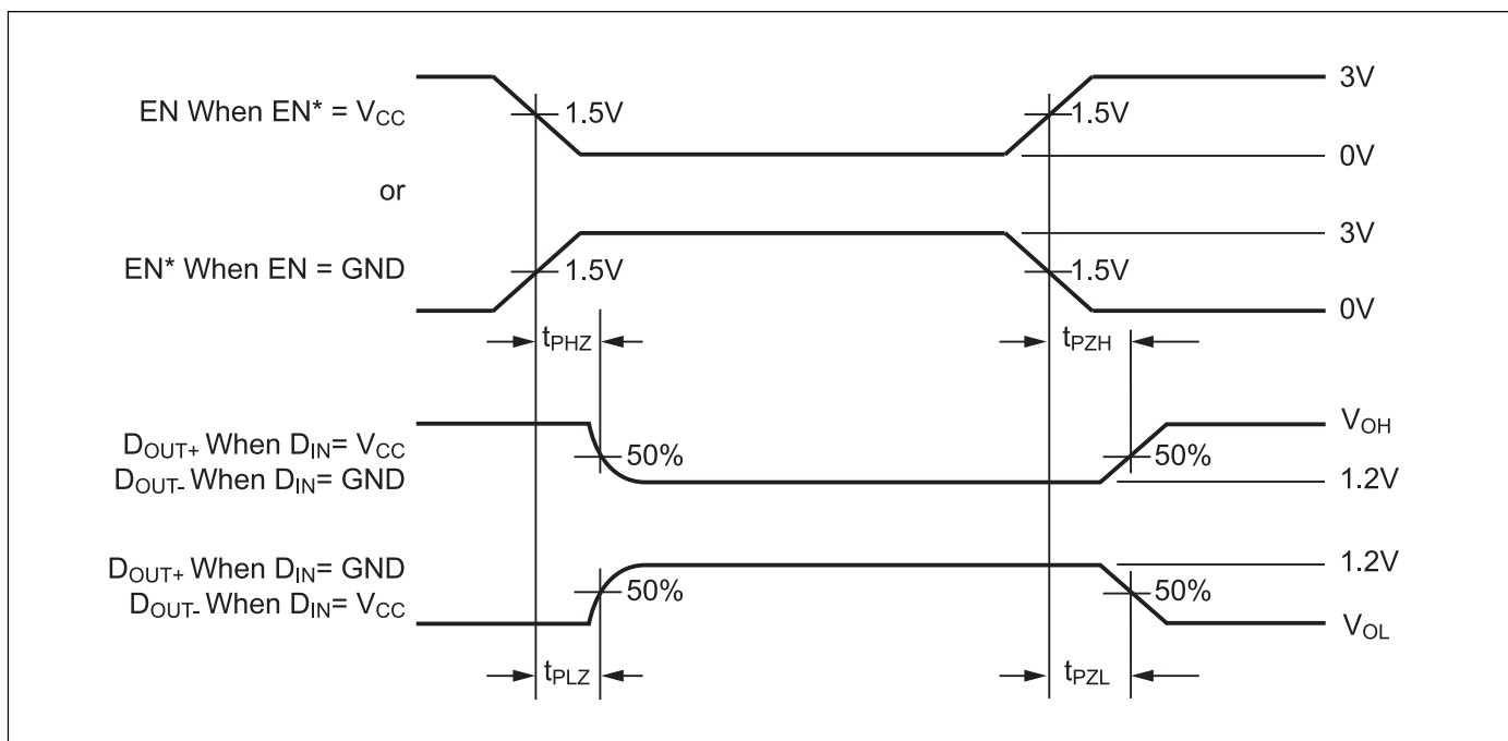
Figure 5. Driver Three-State Delay Waveform
