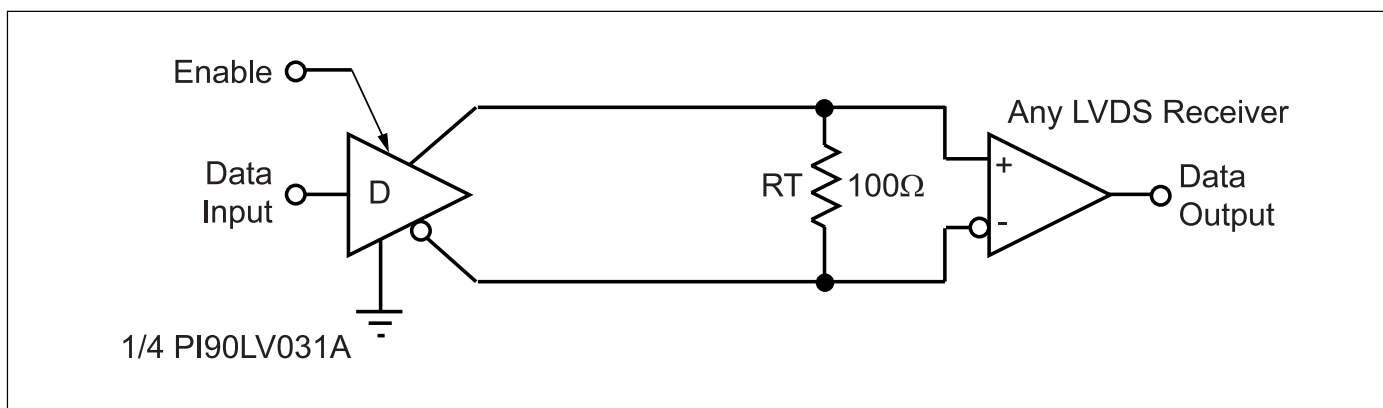
Figure 6. Point-to-Point Application
