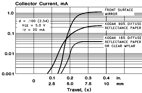
Output Current vs. Position
