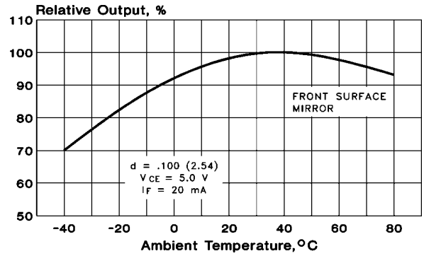
Relative Output vs. Temperature
