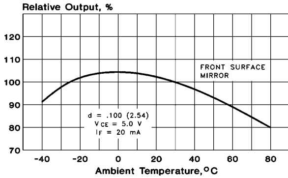
Relative Output vs. Temperature
