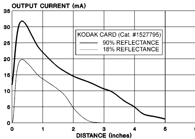
Output Current vs. Sensing Distance
