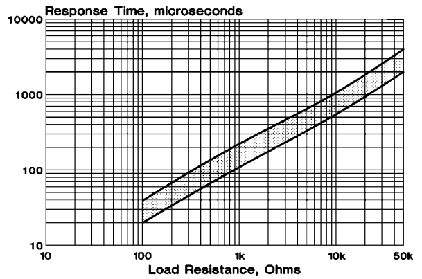
Response Time vs. Load Resistance
