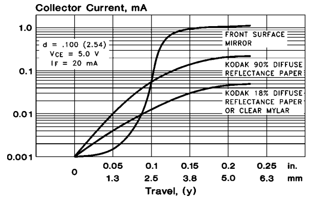
Output Current vs. Position
