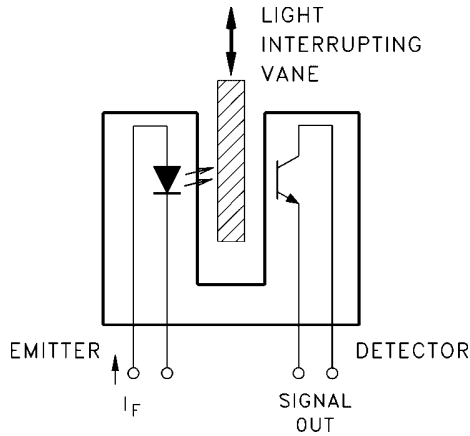
Slotted Switch
