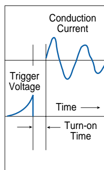
Figure 2. Trigger Voltage Breakdown and Main Gap Conduction Current
