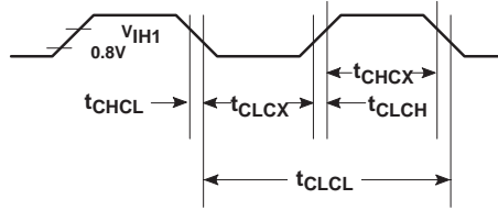
Figure 6. External Clock Drive at XTAL1
