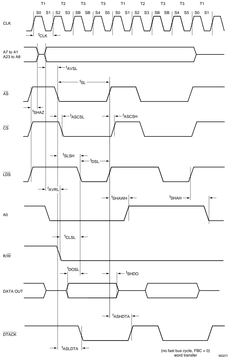
Fig.25 Write cycle timing 8-bit mode clock timing.
