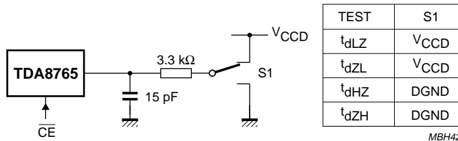
Fig.6 Timing diagram and test conditions of 3-state output delay time.
