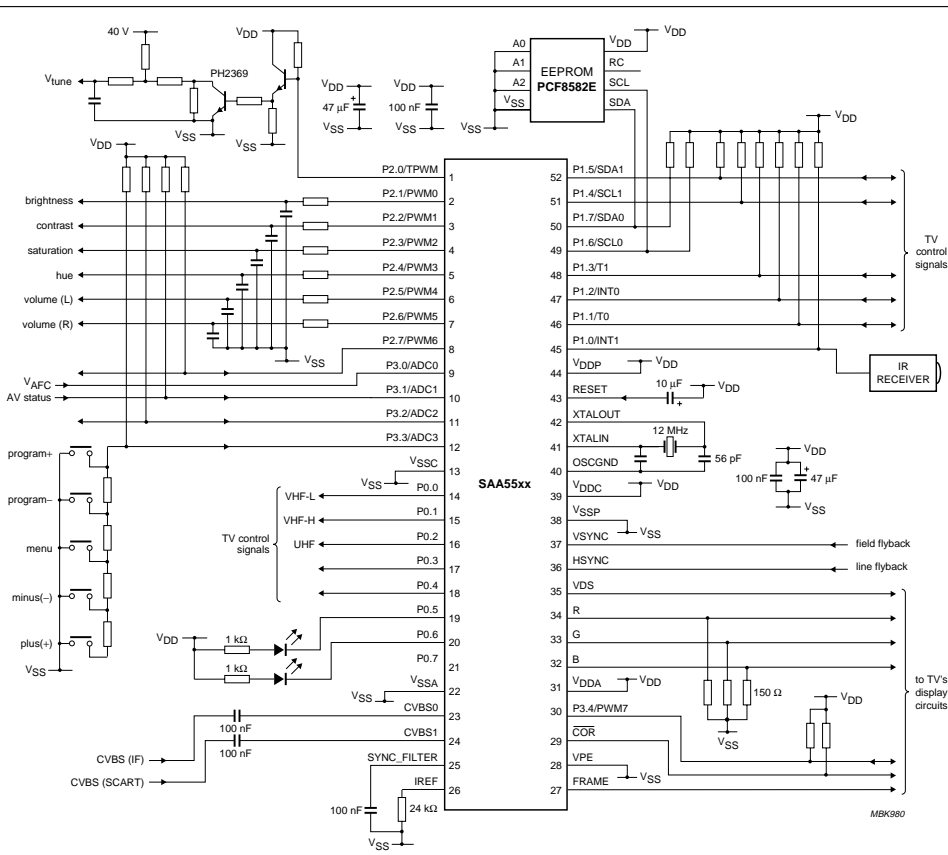
Fig.40 Application diagram.
