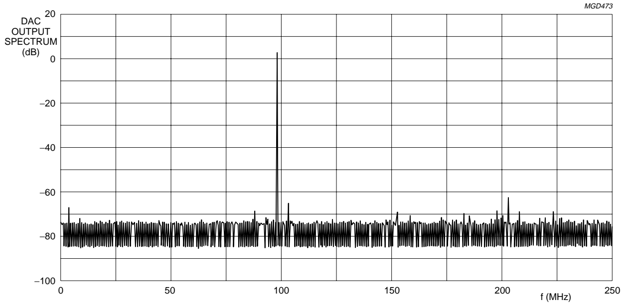
Fig.7 Typical output spectrum; f_{\text{clk}} = 500 \text{ MHz} ; f_{\text{OUT}} = 100 \text{ MHz} .
