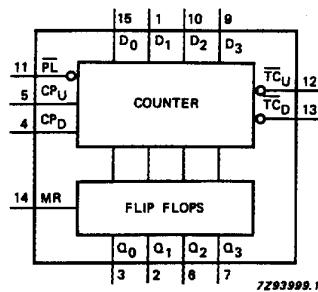
Fig.4 Functional diagram.
