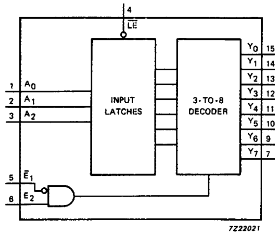
Fig.4 Functional diagram.
