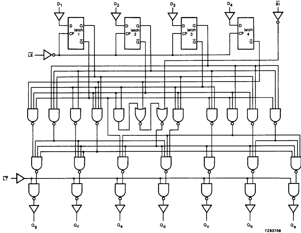
Fig.5 Logic diagram.
