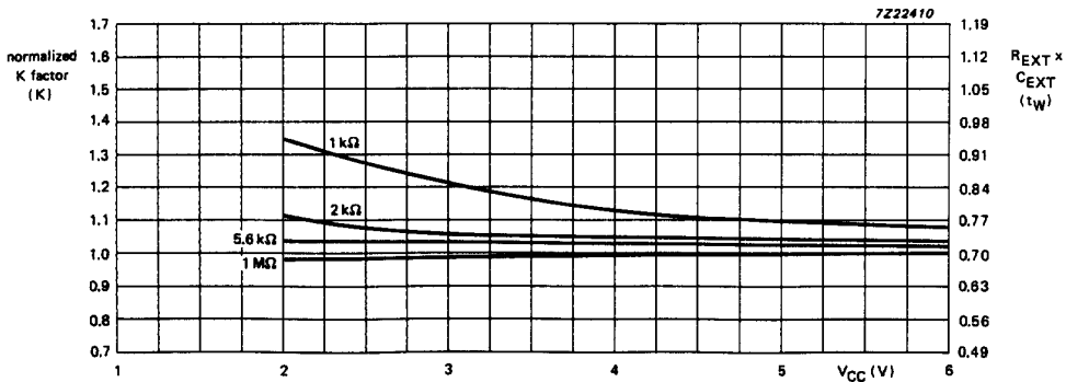
Fig.16 Typical pulse width accuracy versus power supply; C_{EXT} = 100 \text{ nF} ; T_{amb} = 25 \text{ }^\circ\text{C} .
