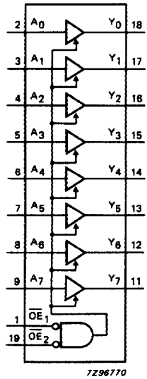
Fig.4 Functional diagram.
