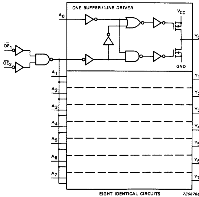
Fig.5 Logic diagram.
