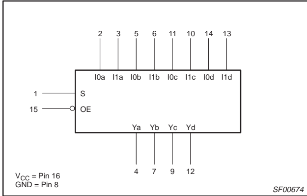
LOGIC SYMBOL – 74ALS257
