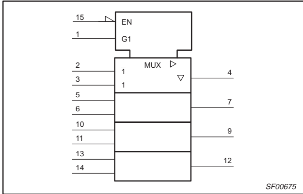
IEC/IEEE SYMBOL – 74ALS257
