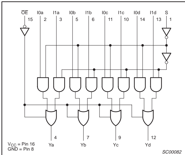
LOGIC DIAGRAM – 74ALS257
