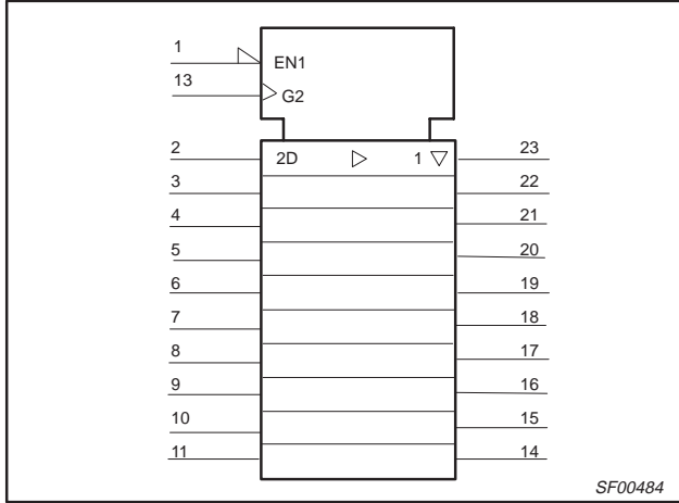
IEC/IEEE SYMBOL – 74F821
