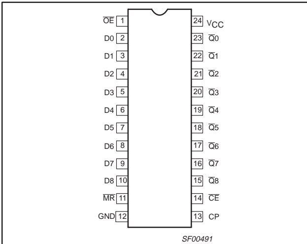
PIN CONFIGURATION – 74F824
