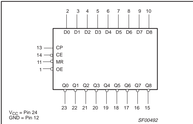
LOGIC SYMBOL – 74F824
