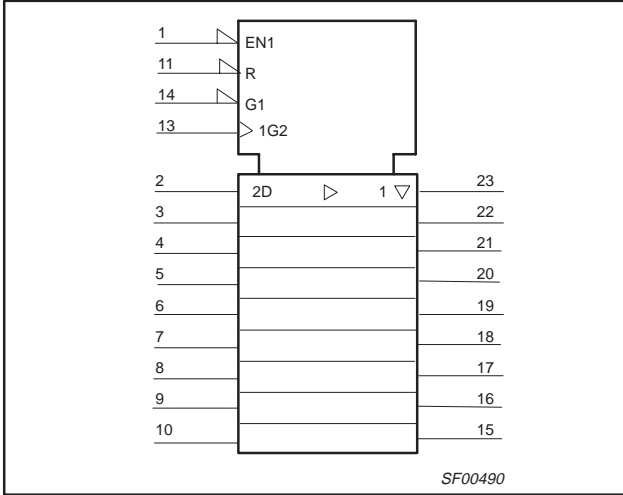
IEC/IEEE SYMBOL – 74F823
