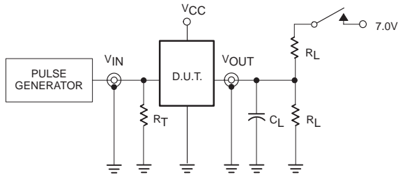
Test Circuit for Open Collector Outputs
