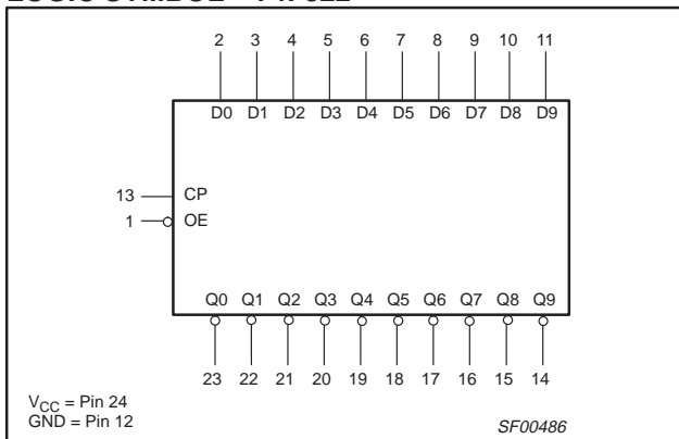
LOGIC SYMBOL – 74F822
