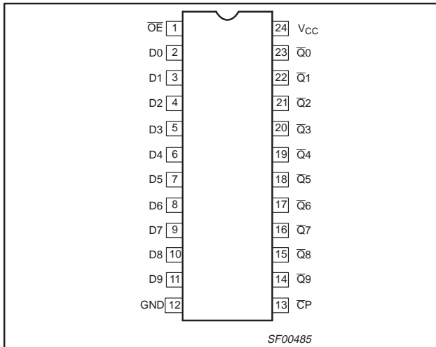
PIN CONFIGURATION – 74F822
