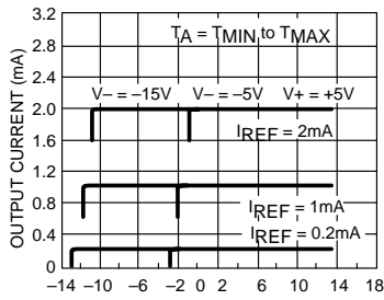
Reference AMP Common-Mode Range All Bits On
