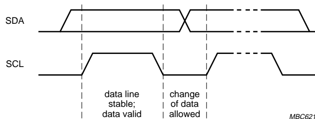
Fig.10 Bit transfer.
