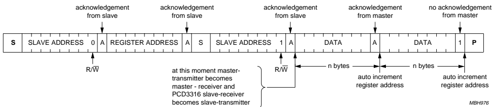
b. I 2 C-bus read sequence.
