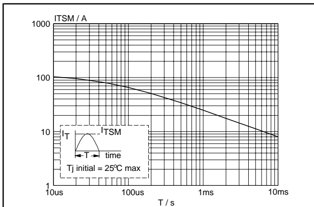
Fig.2. Maximum permissible non-repetitive peak on-state current I_{TSM} , versus pulse width t_p , for sinusoidal currents, t_p \leq 10 ms.
