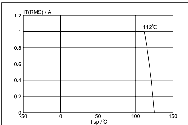
Fig.3. Maximum permissible rms current I_{T(RMS)} , versus solder point temperature T_{sp} .
