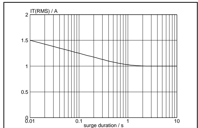
Fig.5. Maximum permissible repetitive rms on-state current I_{T(RMS)} , versus surge duration, for sinusoidal currents, f = 50 Hz; T_{sp} \leq 112^\circ\text{C} .
