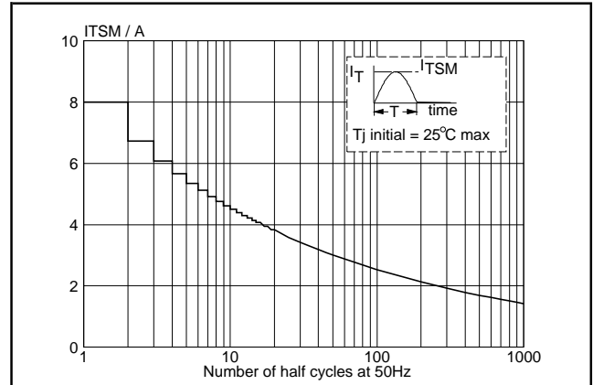
Fig.4. Maximum permissible non-repetitive peak on-state current I_{TSM} , versus number of cycles, for sinusoidal currents, f = 50 Hz.
