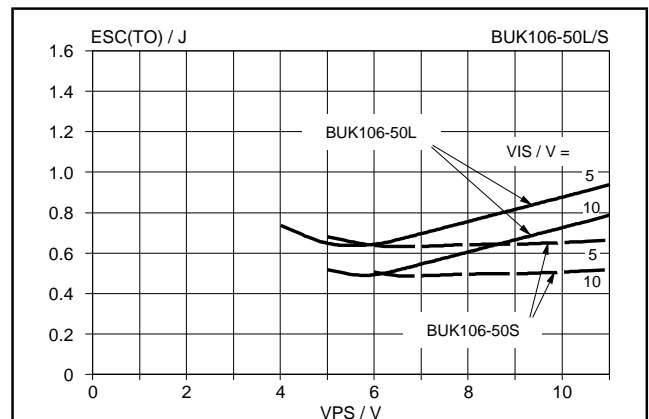
Fig.20. Typical overload protection energy, T_j = 25^\circ\text{C} E_{SC(TO)} = f(V_{PS}); conditions: V_{DS} = 13\text{ V}, parameter V_{IS}
