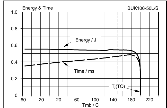
Fig.19. Typical overload protection characteristics. Conditions: V_{DD} = 13\text{ V}; V_{PS} = V_{PSN}; V_{IS} = 8\text{ V}; \text{SC load}
