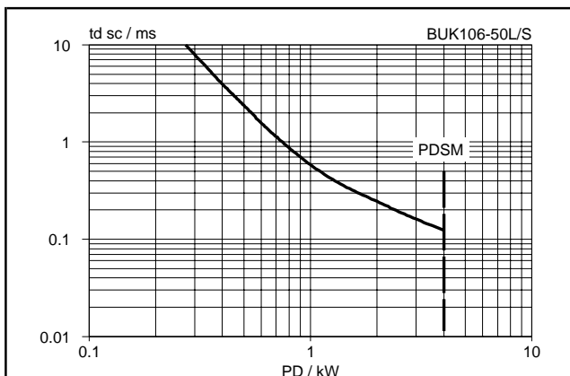
Fig.18. Typical overload protection characteristics. t_{d\text{sc}} = f(P_{DS}); conditions: V_{PS} \geq V_{PSP}; V_{IS} \geq 5\text{ V}
