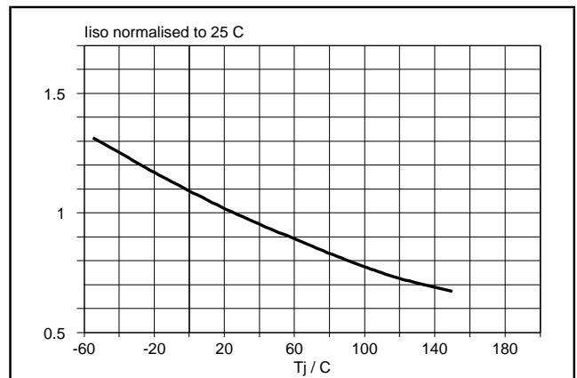
Fig.29. Normalised input current (normal operation). I_{IS}/I_{IS25\ ^\circ\text{C}} = f(T_j); V_{IS} = 10\text{ V}
