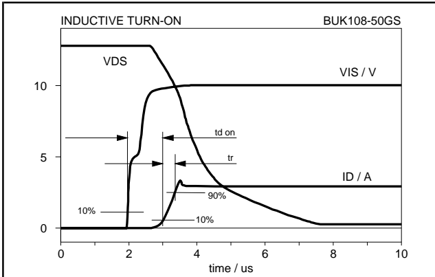
Fig.24. Typical switching waveforms, inductive load. V_{DD} = 13\text{ V}; I_D = 3\text{ A}; R_I = 50\ \Omega, T_j = 25\ ^\circ\text{C}.
