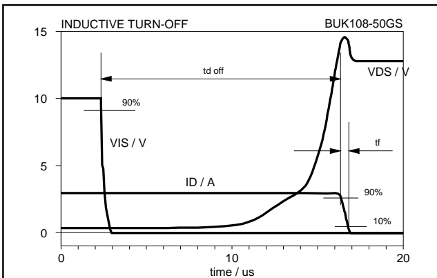
Fig.25. Typical switching waveforms, inductive load. V_{DD} = 13\text{ V}; I_D = 3\text{ A}; R_I = 50\ \Omega, T_j = 25\ ^\circ\text{C}.
