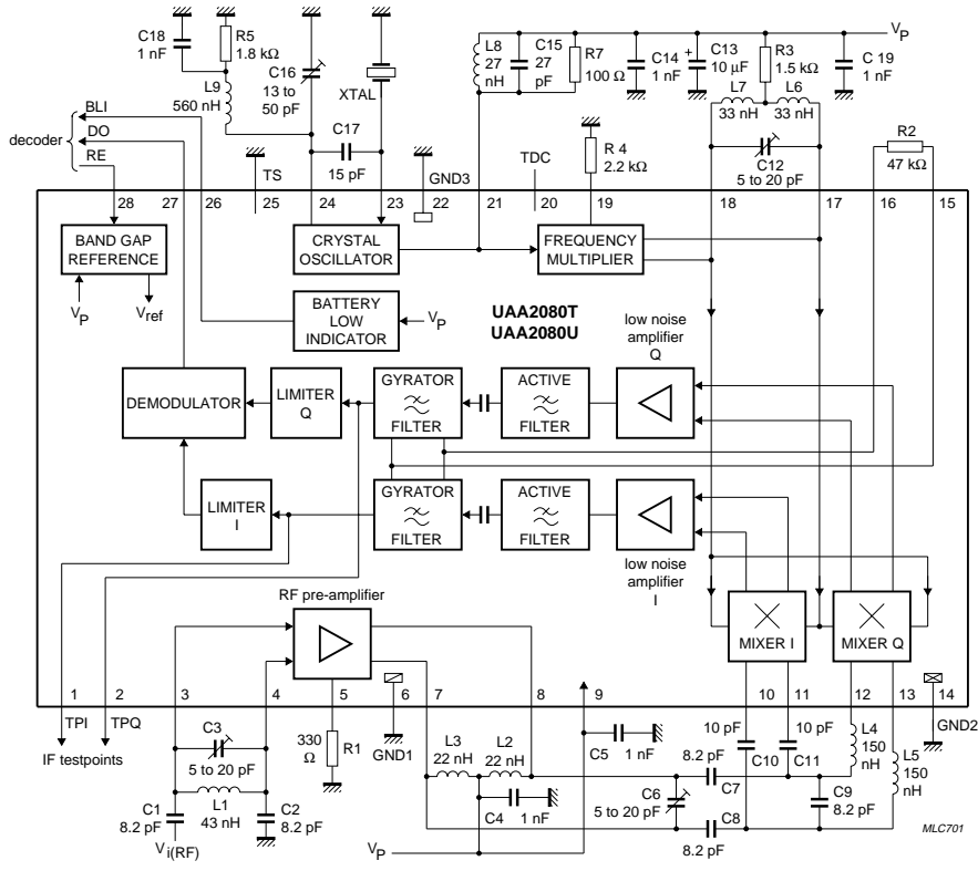
Fig.2 Block, test and application diagram drawn for SO28 and naked die; f_{i(RF)} = 172.941 MHz.
