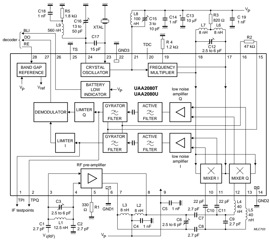
Fig.4 Block, test and application diagram drawn for SO28 and naked die; f_{i(RF)} = 469.95 MHz.
