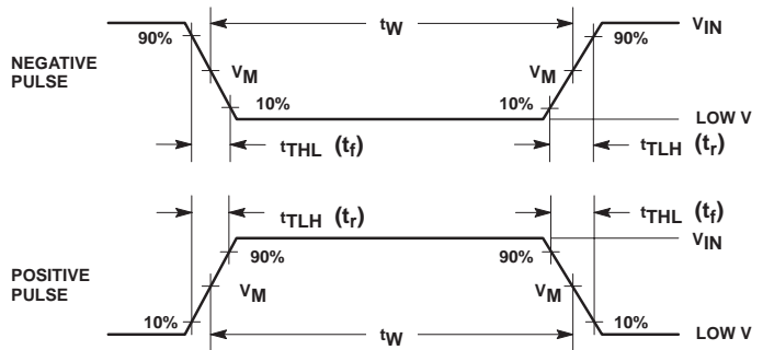
Input Pulse Definitions
