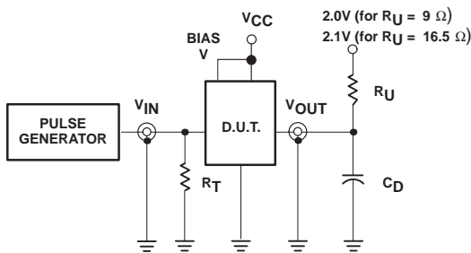
Test Circuit for Outputs on B Port
