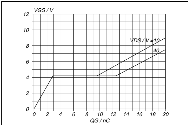
Fig.13. Typical turn-on gate-charge characteristics. V_{GS} = f(Q_G) ; conditions: I_D = 20\text{ A} ; parameter V_{DS}
