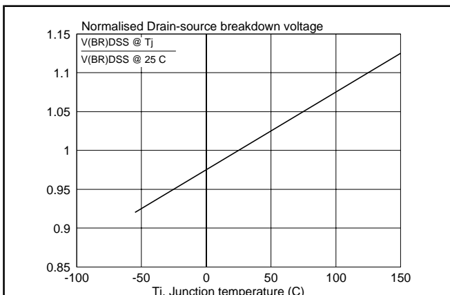
Fig.15. Normalised drain-source breakdown voltage. V_{(BR)DSS @ T_j} / V_{(BR)DSS @ 25 C} = f(T_j)
