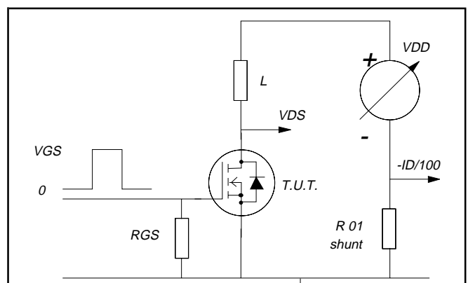
Fig.18. Unclamped inductive test circuit.
