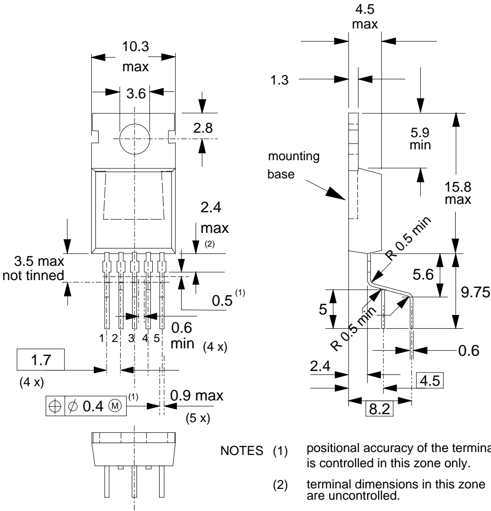
Fig.38. SOT263 leadform 263-01; pin 3 connected to mounting base.
