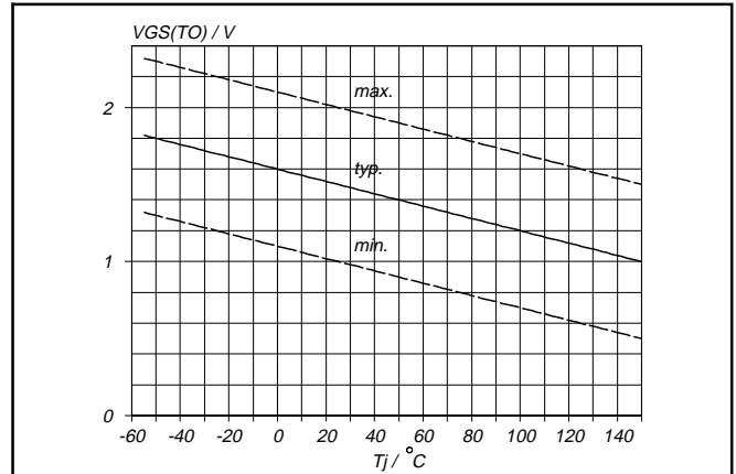
Fig. 10. Gate threshold voltage. V_{GS(TO)} = f(T_j) ; conditions: I_D = 0.1 mA; V_{DS} = V_{GS}
