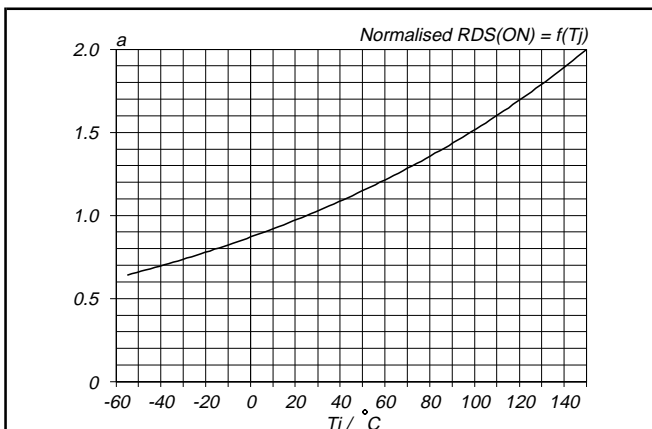
Fig. 9. Normalised drain-source on-state resistance. a = R_{DS(ON)} / R_{DS(ON)25^{\circ}C} = f(T_j) ; I_D = 0.9 A; V_{GS} = 5 V
