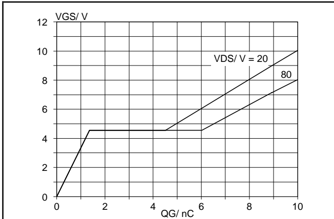
Fig.13. Typical turn-on gate-charge characteristics. V_{GS} = f(Q_G) ; conditions: I_D = 1.8 A ; parameter V_{DS}
