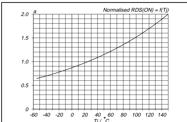
Fig. 9. Normalised drain-source on-state resistance. a = R_{DS(ON)}/R_{DS(ON)25\text{ °C}} = f(T_j) ; I_D = 1.8\text{ A} ; V_{GS} = 10\text{ V}
