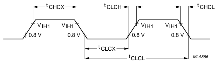
Fig.47 External clock drive XTAL1.
