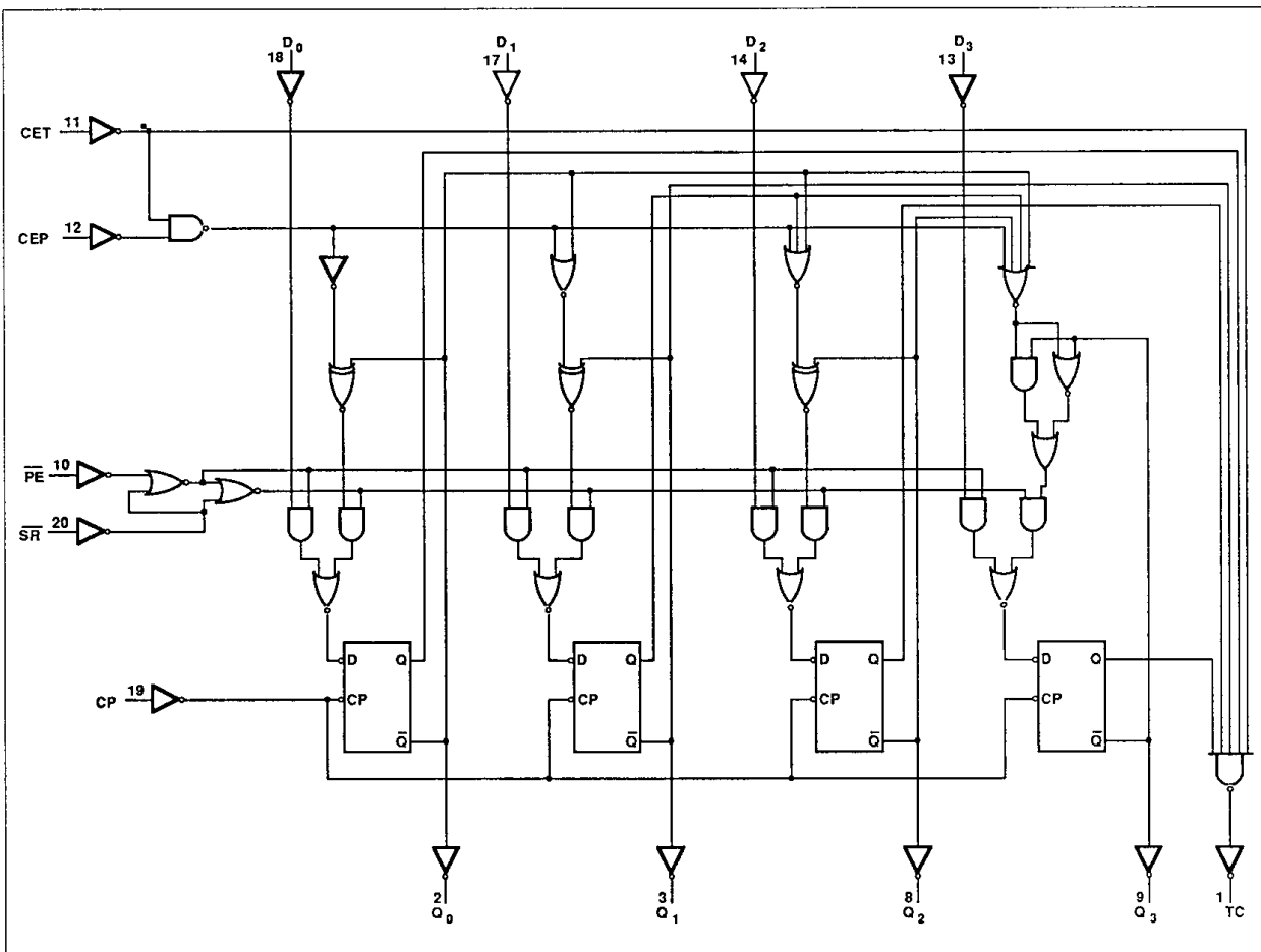
LOGIC DIAGRAM
