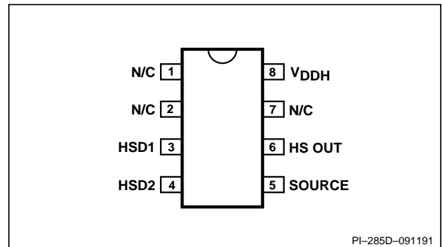
Figure 2. Pin Configuration.
