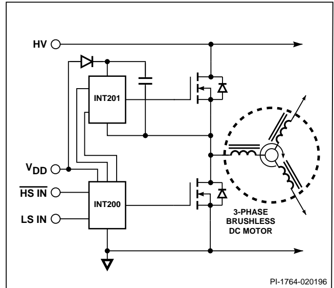
Figure 1. Typical Application.
