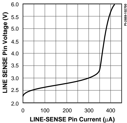
Figure 62a. LINE-SENSE Pin Voltage vs. Current.
