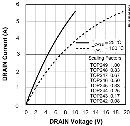
Figure 66. Output Characteristics.
