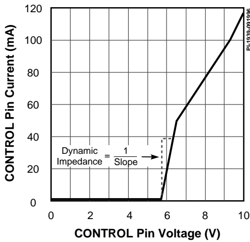
Figure 51. CONTROL Pin I-V Characteristic.
