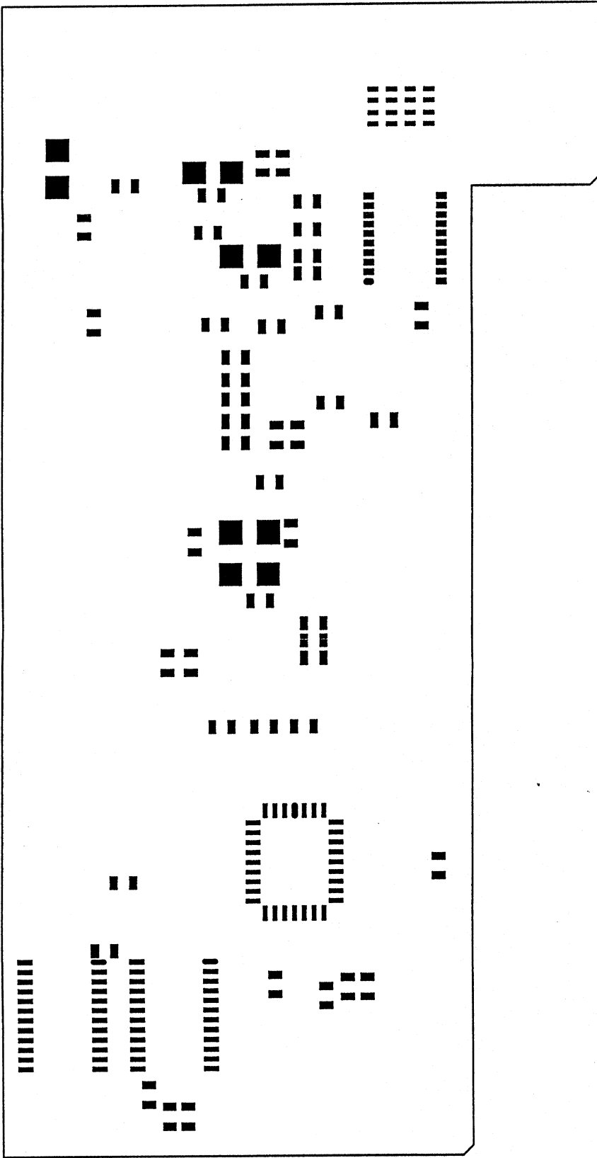
UTP5_1-1 Bottom Paste Mask
