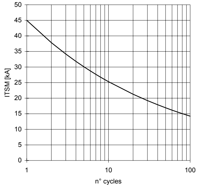
SURGE CHARACTERISTIC T_j = 175^\circ\text{C}
