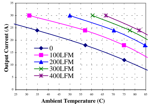
Fig.10 QLS30ZB (1.8V) derating curves
