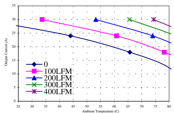
Fig.11 QLS30ZA (1.5V) derating curves
