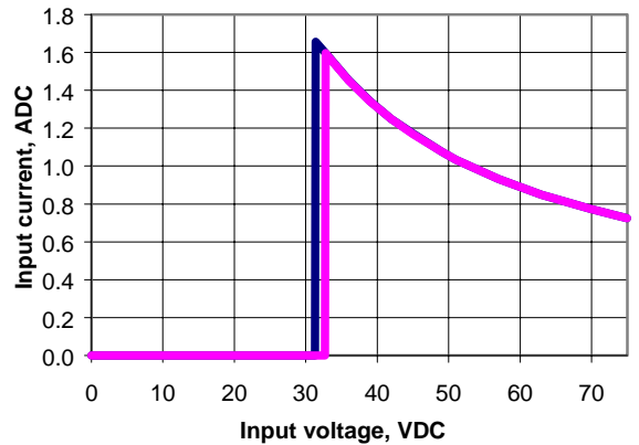
Fig. 5 QLS30ZA Input Characteristic
