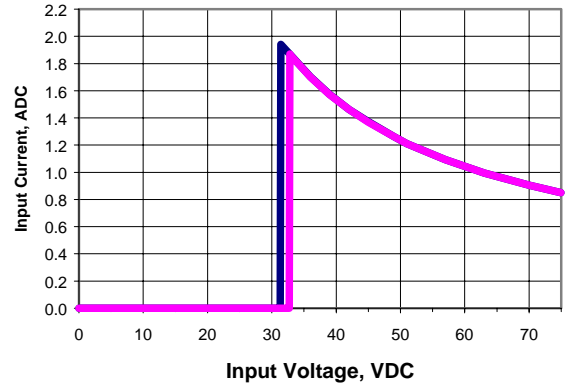
Fig. 4 QLS30ZB Input Characteristic
