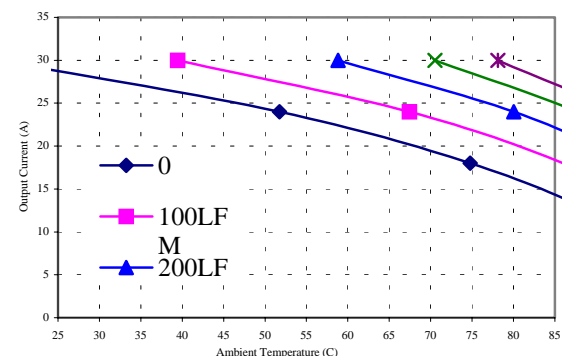
Fig.12 QLS30ZY (1.2V) derating curves
