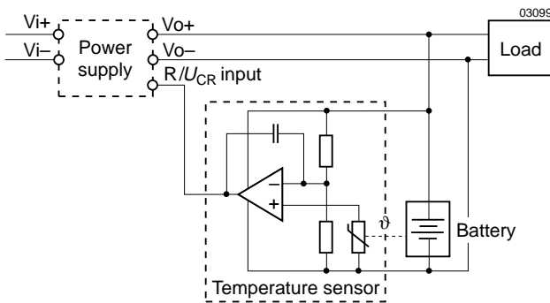
Fig. 2 Functional description
