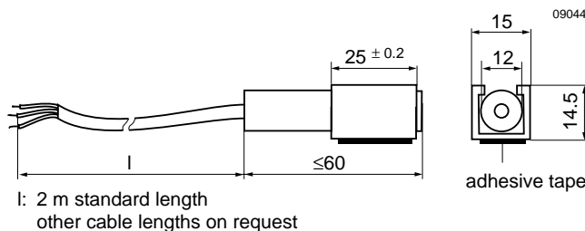
Fig. 5: T and U temperature sensor with mounting fixture.
