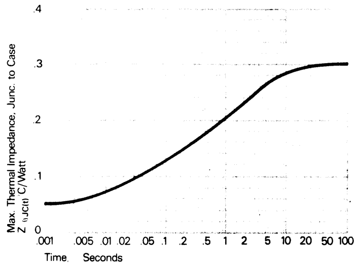
Figure 5. Transient thermal impedance versus time.
