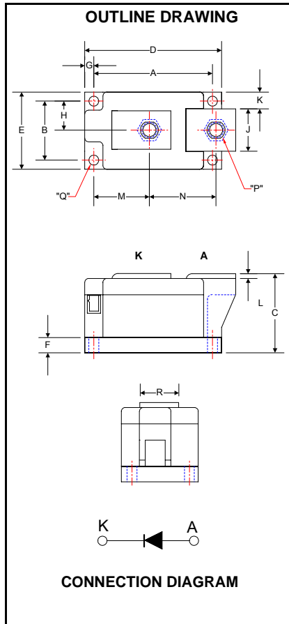
LS41__60 Single Diode POW-R-BLOK™ Module 600 Amperes / 800-2400 Volts
