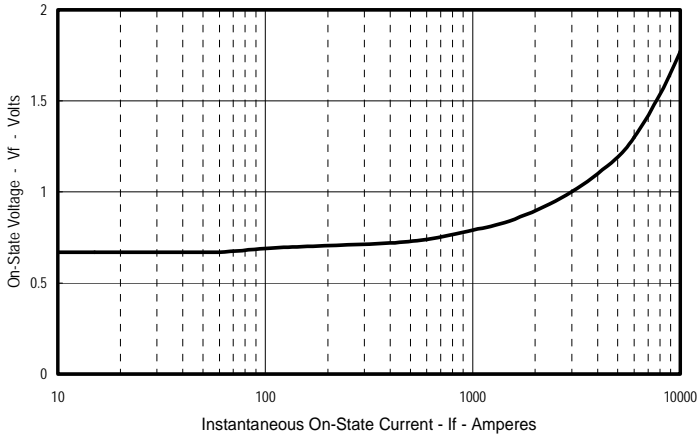
Typical On-State Forward Voltage Drop (Tj = 150C)
