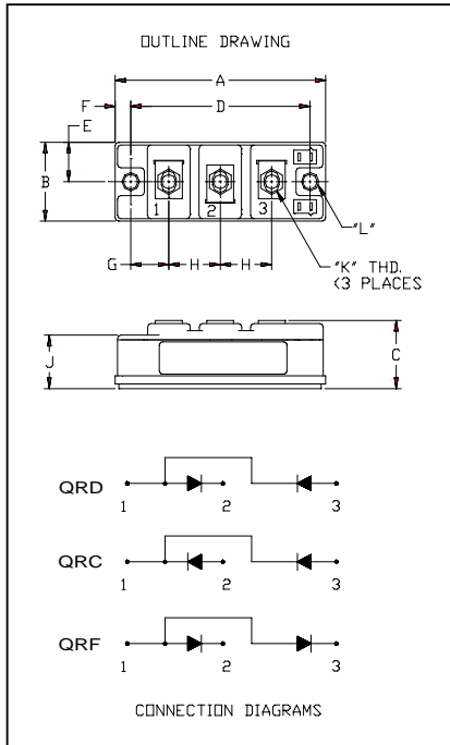
QR_0640T30 Fast Recovery Diode Module 400 Amperes / 600 Volts
