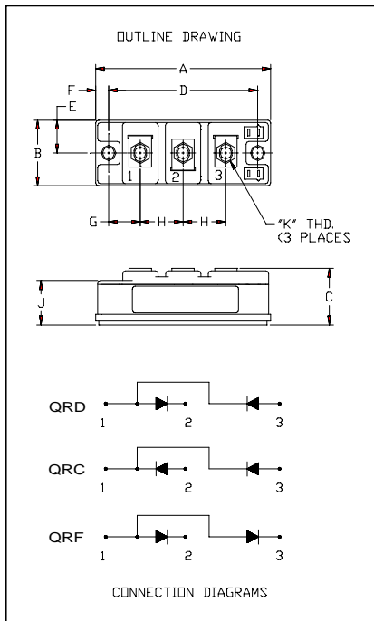
QR_1210T30 Fast Recovery Diode Module 100 Amperes / 1200 Volts
