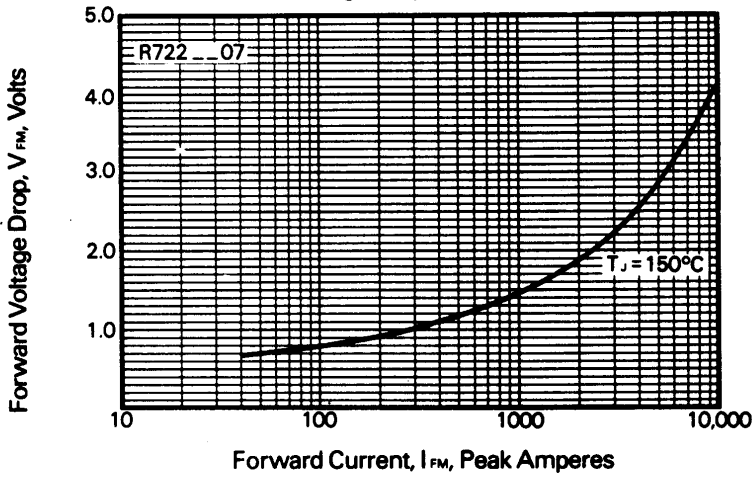
Forward Voltage Drop vs. Forward Current
