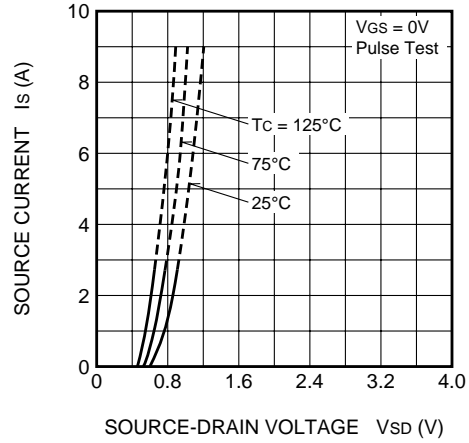
SOURCE-DIODE FORWARD CHARACTERISTICS (TYPICAL)
