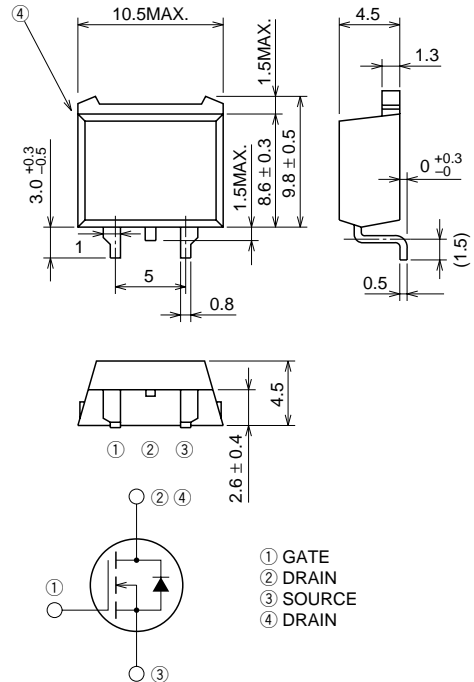
TO-220S
